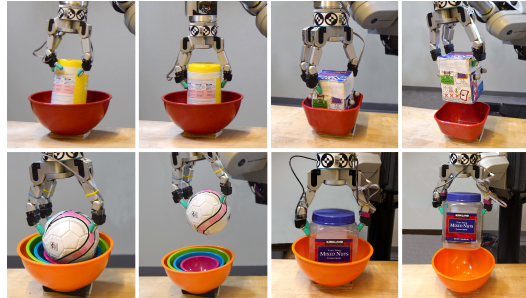
Fig. 1: Objects and experimental setup used for learning the grasp stability predictor and the regrasping behavior. Top-left : the cylinder. Top-right : the box. Bottom-left : the ball. Bottom-right : the novel object.
